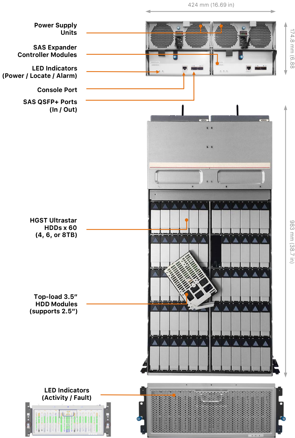
Rear View
